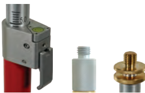
QLV lock body Fixed Tip Adjustable Tip
